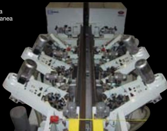
Sanding machine, double version for simultaneous sanding of the two edges.
